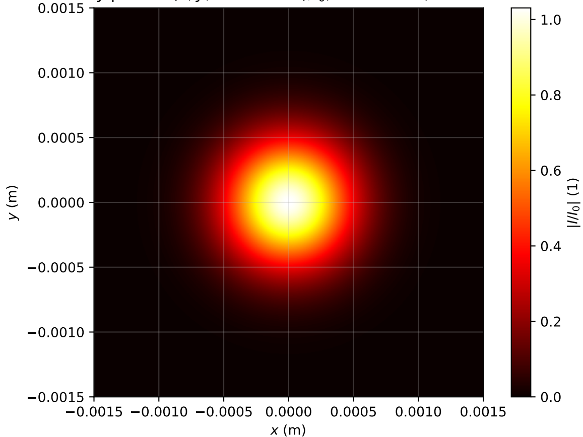
Intensity profile I(x, y, z = 0.239m)/I_0 , \text{Pin}=0.8\text{Pcr} , artificial time
